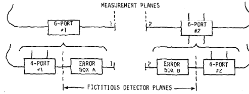
Fig. 3. The six-port reflectometer may also be reduced to an ideal four-port in cascade with an "error box."
