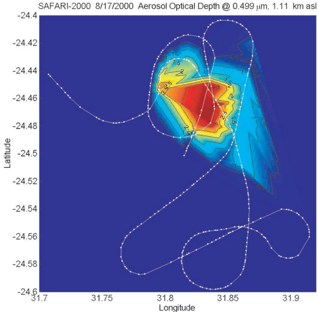
Figure 5. Map of \tau_a(0.499 \mu\text{m}) of a smoke plume originating from a flaming-hot grass fire on 17 August 2000, in the Kruger National Park North of Skukuza ( 24^{\circ}28'S/31^{\circ}50'E ). The \tau_a(\lambda) measurements are taken at each individual white dot along the white Convair-580 flight track. A triangle-based linear interpolation is used to fill in \tau_a values between the flight tracks. Size of the map is 22.25 \times 22.25 \text{ km}^2 .
