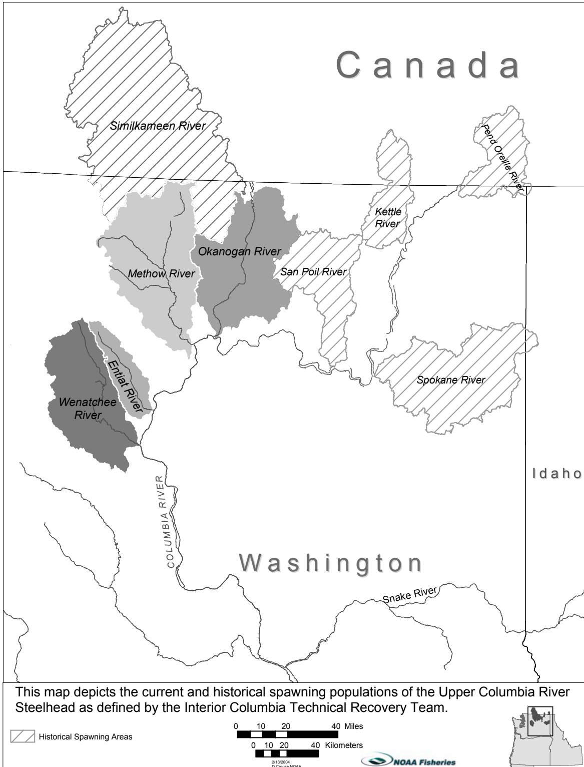
Figure B-7. Historical spawning populations of the Upper Columbia River Steelhead.
