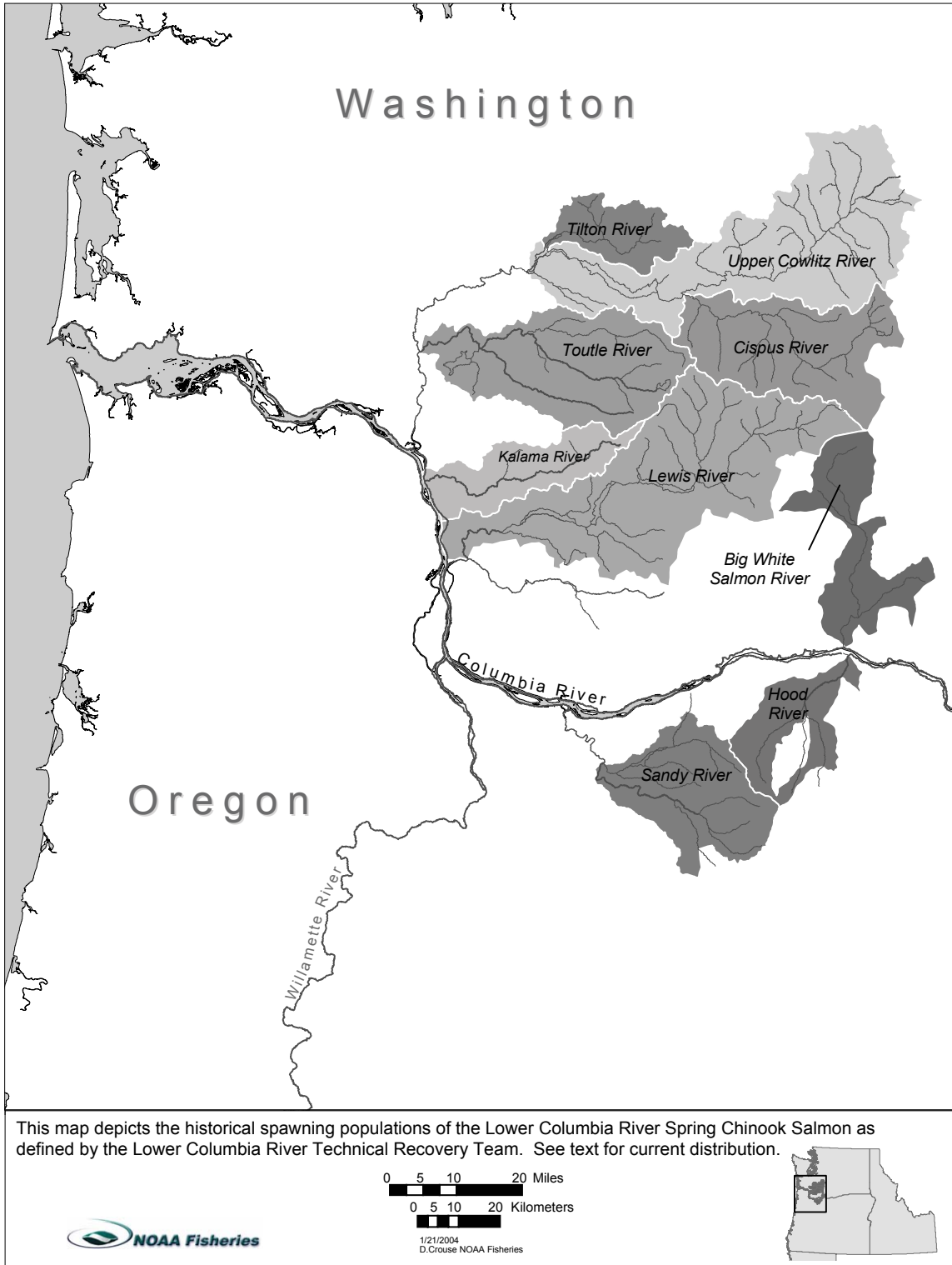
Figure B-5b. Historical spawning populations for the Lower Columbia River Spring Chinook Salmon.
