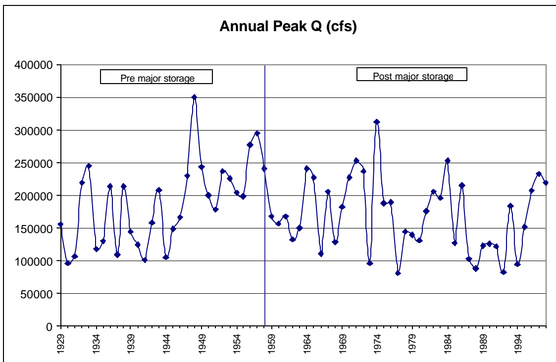
Figure 4-17. Lower Snake River Annual Peak Discharge, 1929 to 1998
