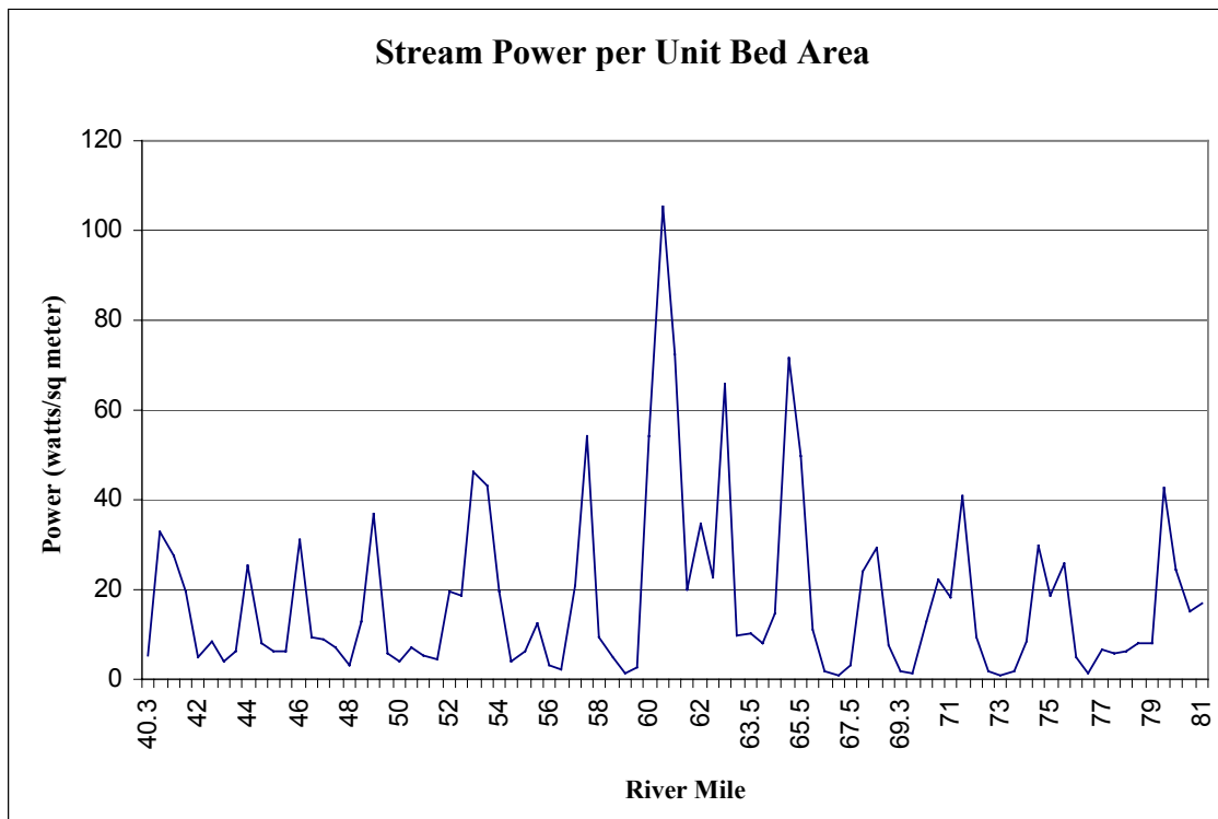
Figure 4-11. Stream Power at Each Cross Section for Q_{50} Flow
