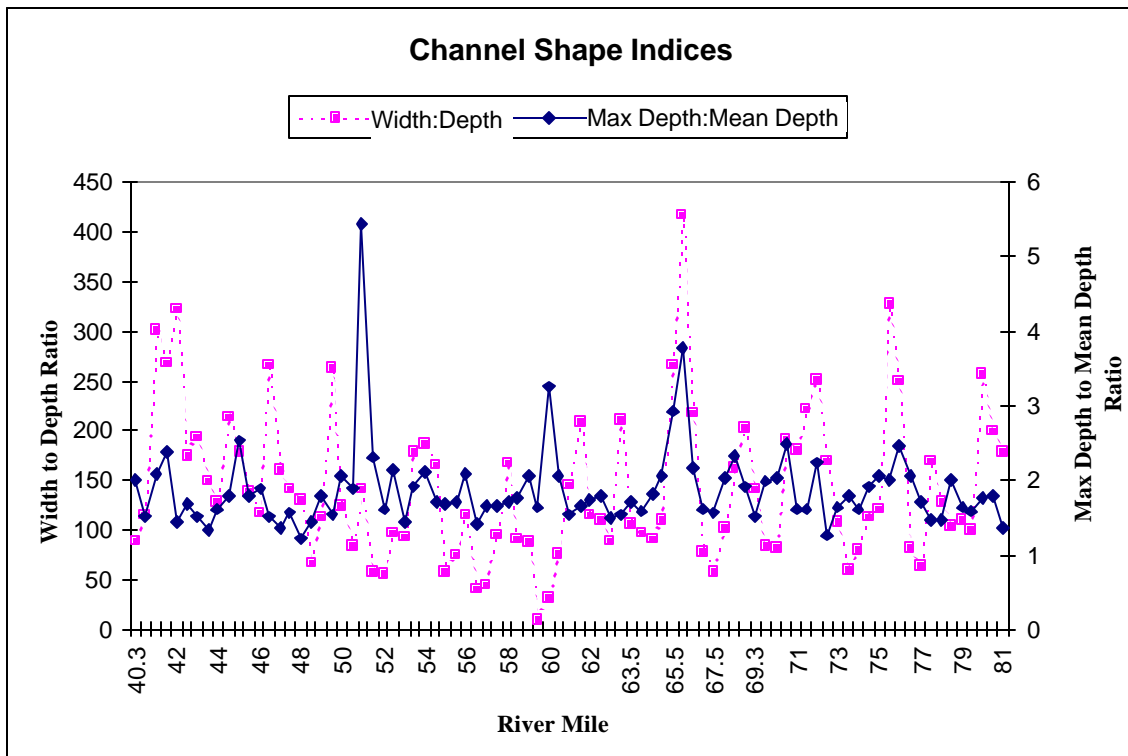
Figure 4-14. Channel Shape Indices at Each Cross Section for Q 50 Flow
