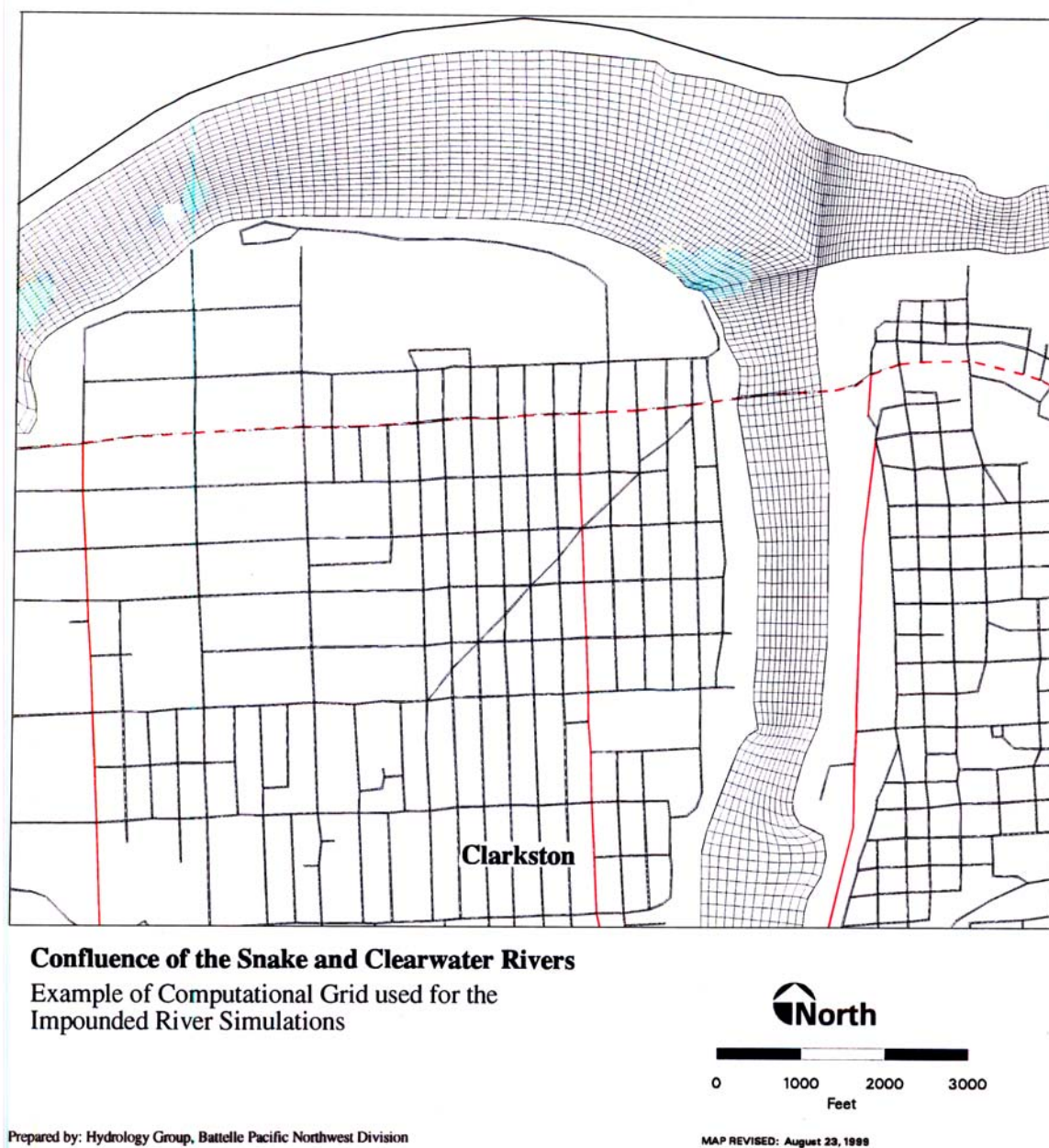
Figure 8-1. Example of the Computational Grid Used in the Full-pool, Impounded Conditions Simulations
