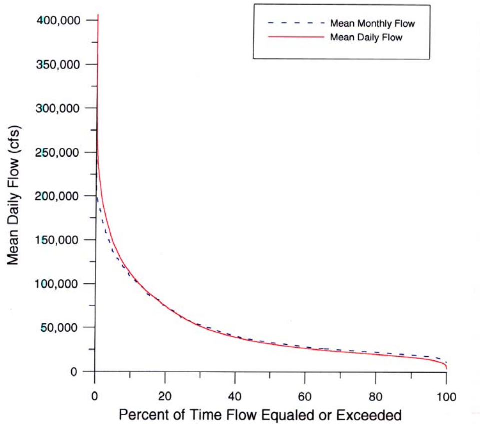
Figure 8-3. Flow Duration Curves Based on Mean Monthly and Mean Annual Flows at Lower Granite Dam
