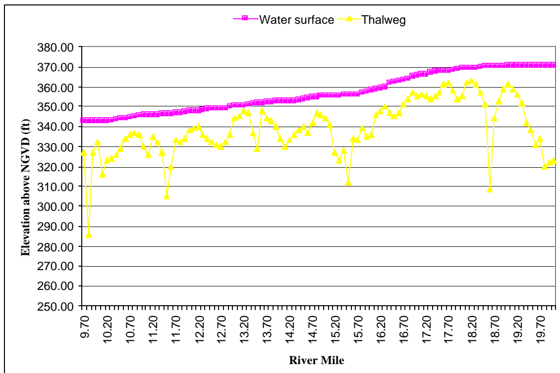
Figure 4-12. Longitudinal Profile of Water Surface and Thalweg Elevations for Q_{90} Flow Note: NGVD=National Geodetic Vertical Datum
