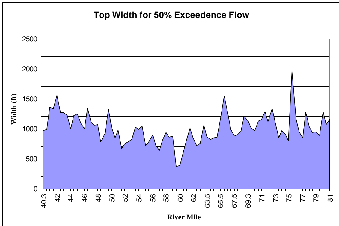
Figure 4-15. Top Width at Each Cross Section for Q_{50} Flow
