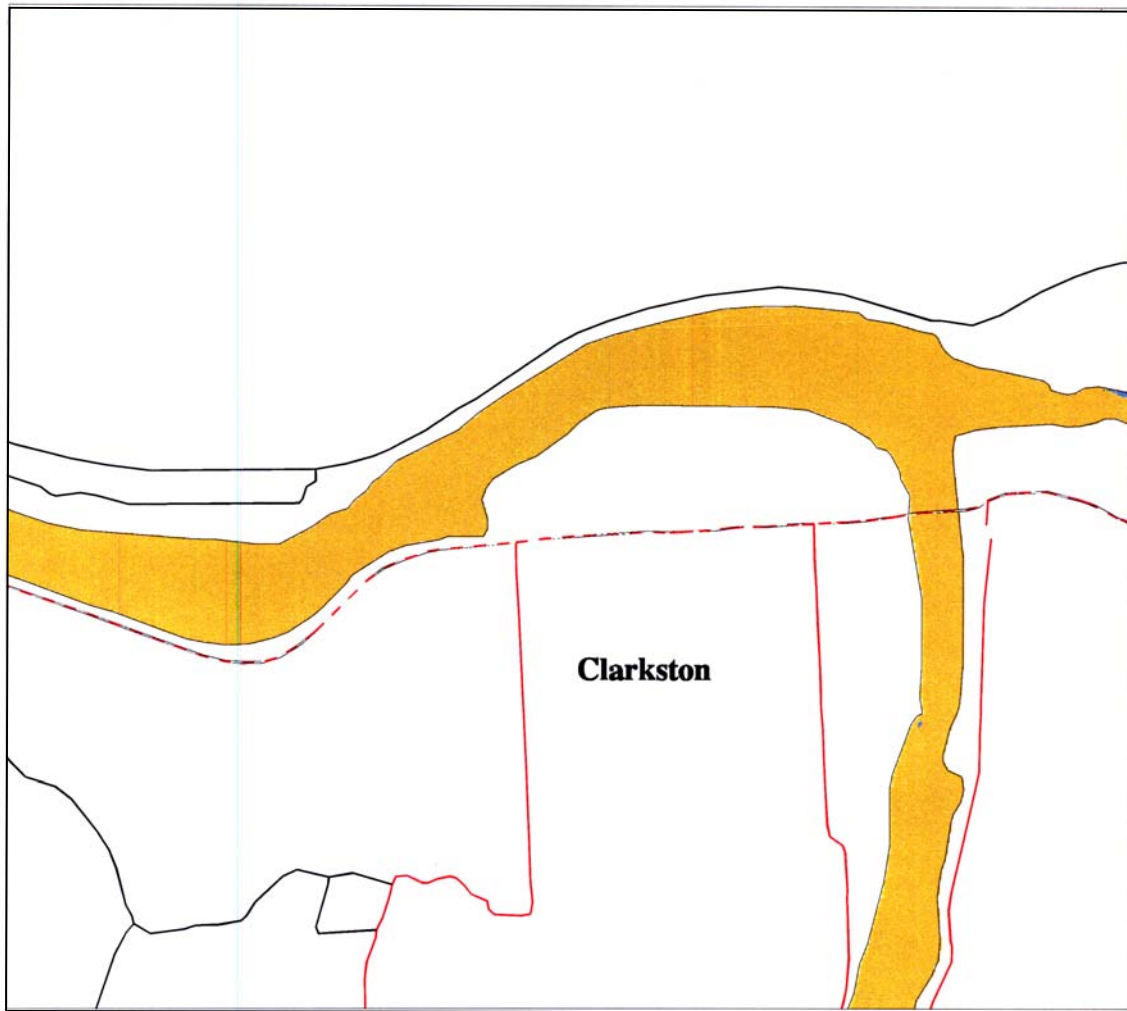
Confluence of the Snake and Clearwater Rivers Fall Chinook Spawning Habitat Suitability for the Impounded River for the 50 Percent Exceedance Flow 31710 cfs
