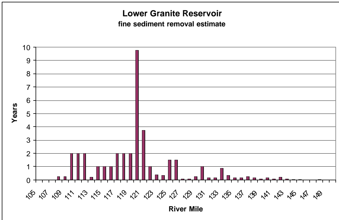
Figure 4-18. Estimated Time to Remove Fine Sediments From Lower Granite Reservoir Under Dam Breaching
