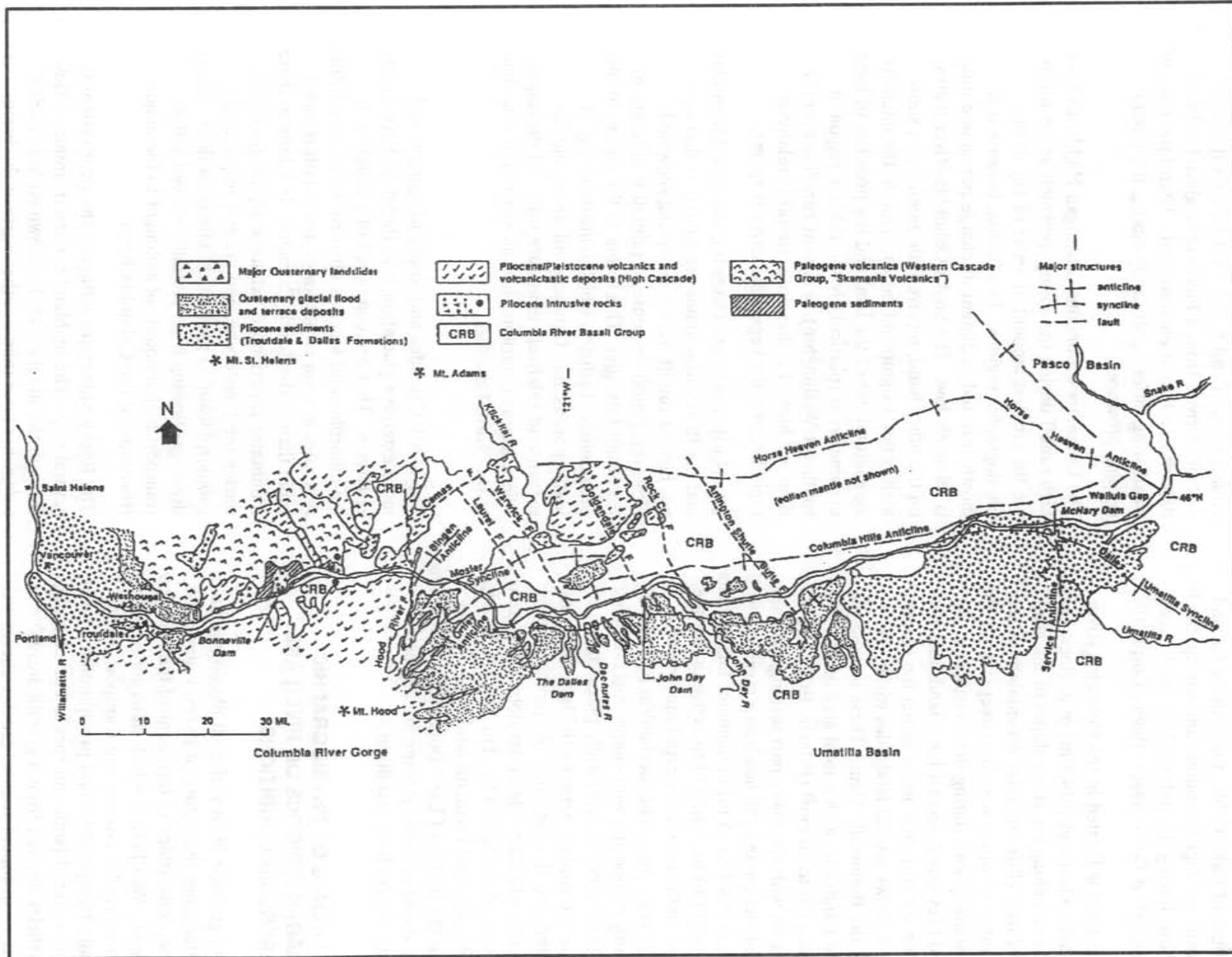
Figure 2-4. Generalized Geologic Map of the Area Along the Lower Columbia River.
