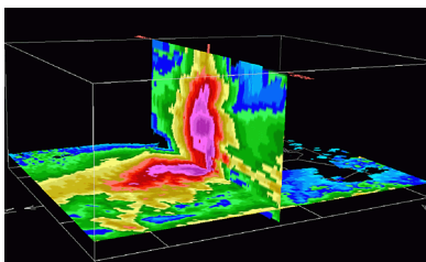
Vertical cross-section of reflectivity on a composite reflectivity layer.
