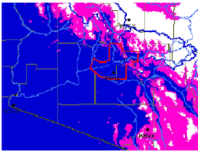
Precipitation phase product using RUC-2 model 0C heights
