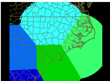
QPE-SUMS uses a mosaic of radar data based on the best available coverage above ground.
