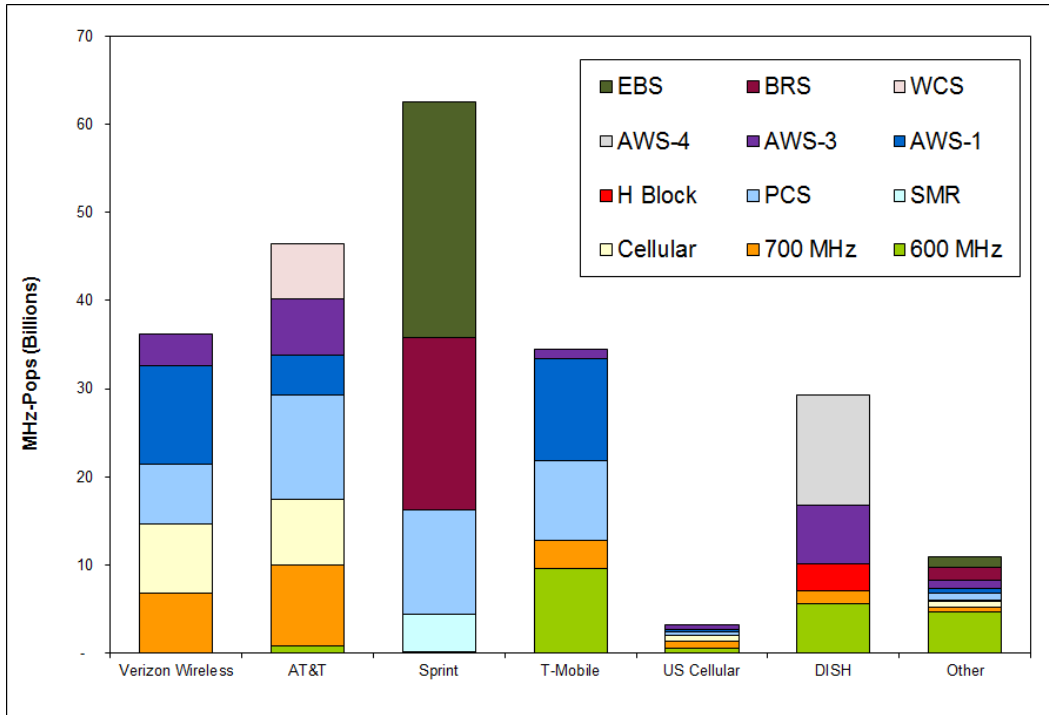
Fig. A-26: Spectrum Holdings by Band Weighted by Population
