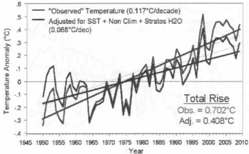
Figure 7. Annual global average temperature history from 1950 to 2009 (source: U.K. Hadley Center) and adjusted annual global average temperature to remove SST errors (Thompson et al., 2008), non-climatic influences (McKittrick and Michaels, 2007) and the influence of stratospheric water vapor increases (Solomon et al., 2010).
