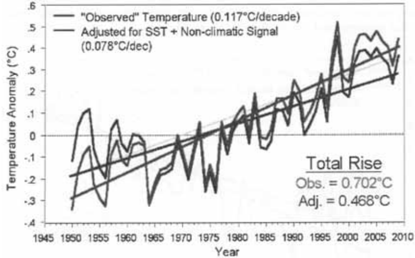
Figure 6. Annual global average temperature history from 1950 to 2009 (source: U.K. Hadley Center) and adjusted annual global average temperature to remove SST errors (Thompson et al., 2008) and non-climatic influences (McKittrick and Michaels, 2007).
