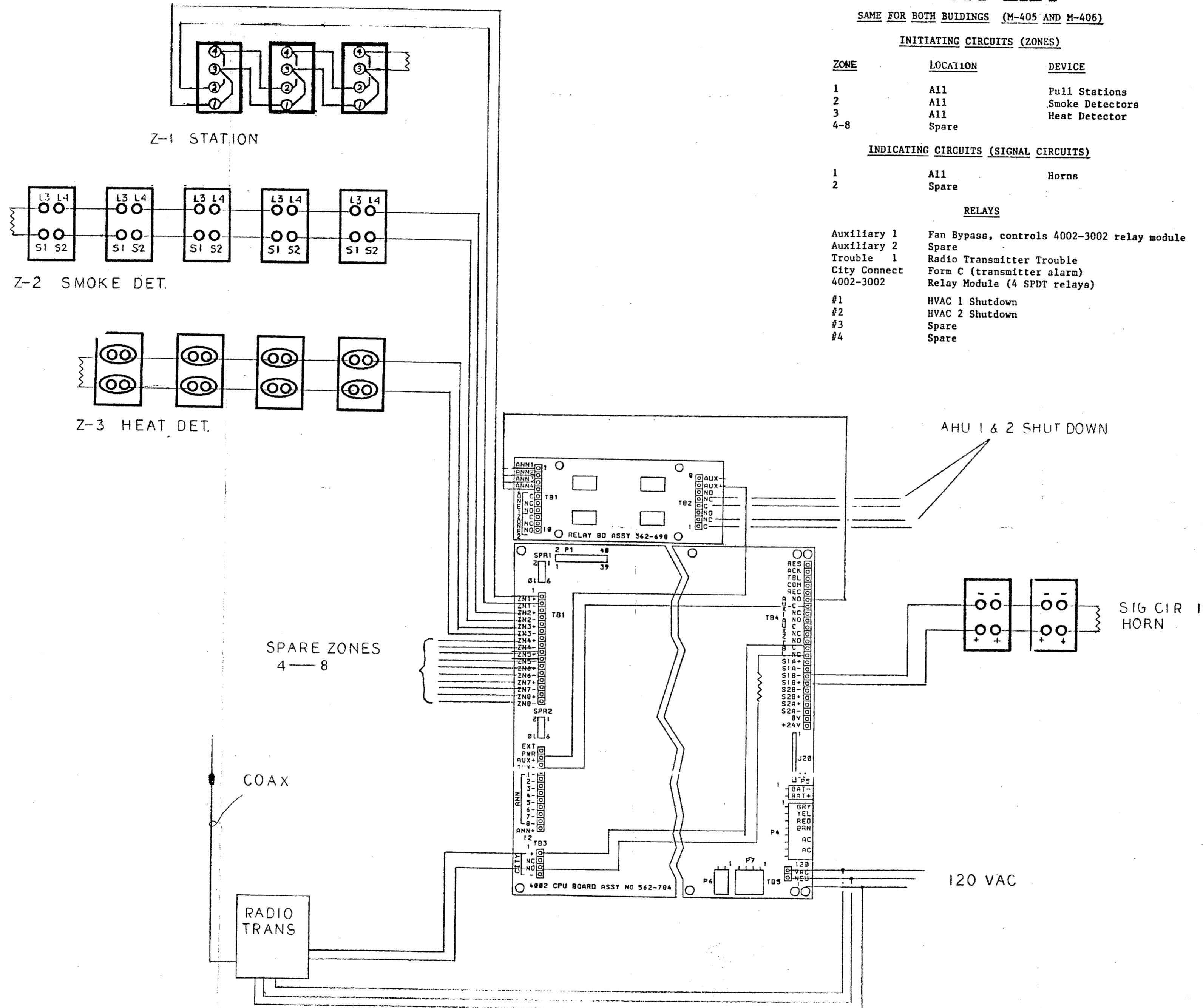
FIRE ALARM SYSTEM RISER DIAGRAM
