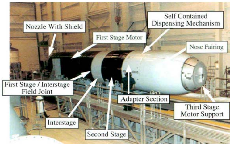
Missile Loaded on a Bare Missile Bridge
