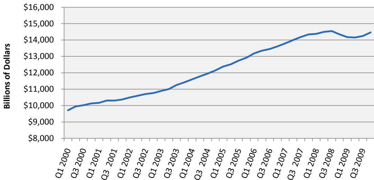
Figure 51: GDP
