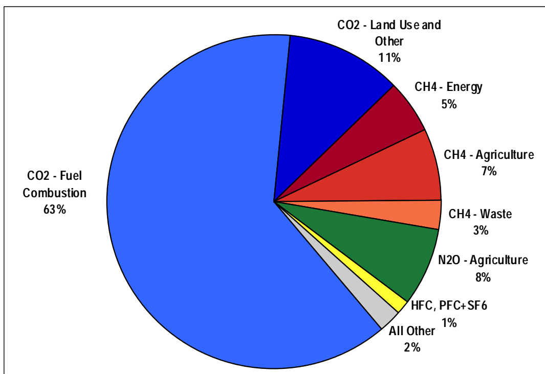
Figure 1. Estimated Sectoral and Greenhouse Gas Shares of Global Emissions in 2005
