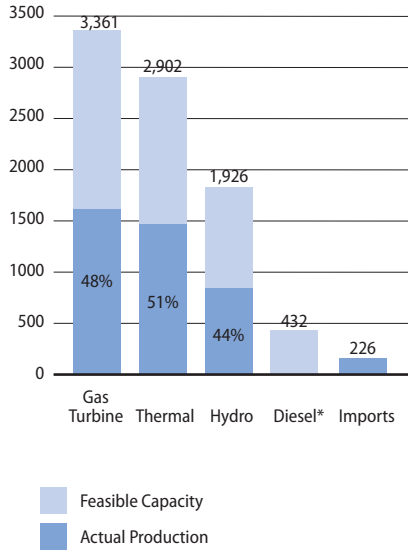
Figure 2-10 ACTUAL PRODUCTION VS. FEASIBLE ELECTRICITY CAPACITY Megawatts (MW) Source: IRMO, Daily Electricity Report (1/1/2007 - 3/31/2007)
